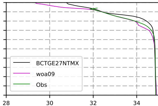
1976 mean Salinity @ moor Arctic B box
