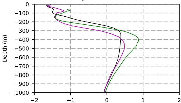
1976 mean temperature @ moor Arctic B box
