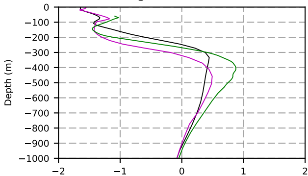
1977 mean temperature @ moor Arctic B box
