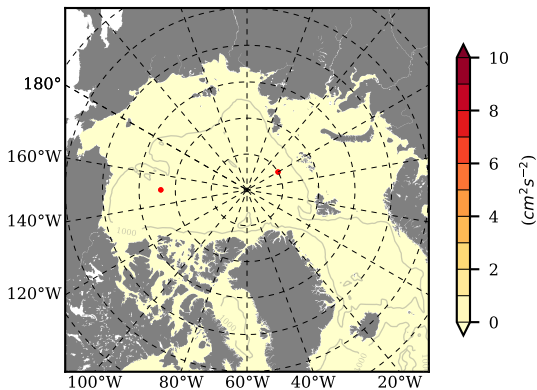
BCTGE28 mean EKE @ 0 m over 2013
