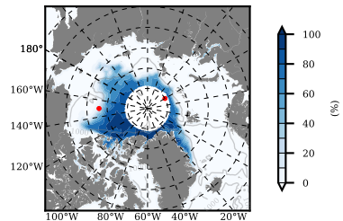
NSIDC mean SICON m09 2010
