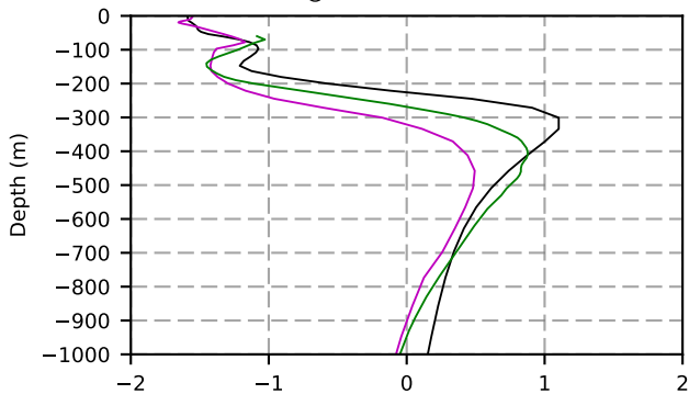
2010 mean temperature @ moor Arctic B box
