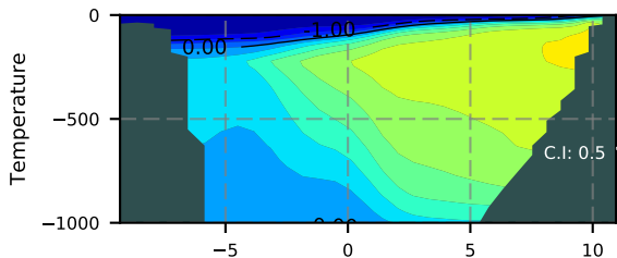
BCTGE28 / FramS Section 1992
