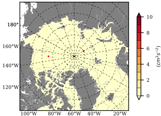
BCTGE28ERA5SC1BDY mean EKE @ 0 m over 1992
