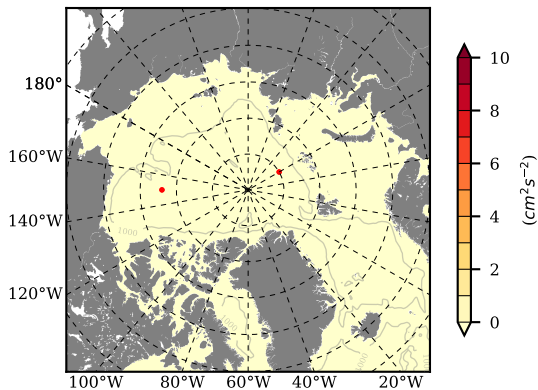
BCTGE28ERA5SC1BDY mean EKE @ 0 m over 1994
