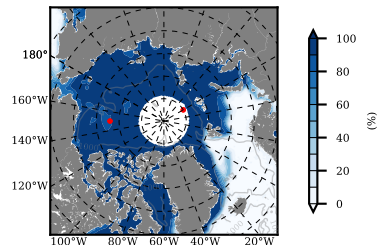
NSIDC mean SICON m09 1988
