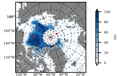
NSIDC mean SICON m09 2012
