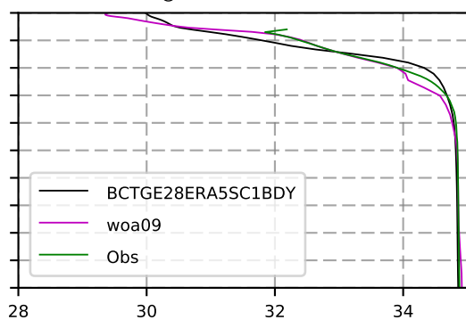
2017 mean Salinity @ moor Arctic B box
