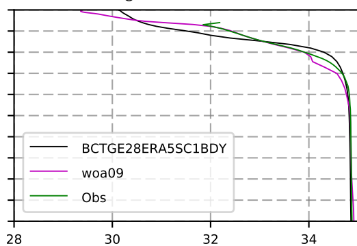
2018 mean Salinity @ moor Arctic B box
