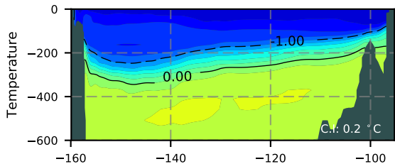
BCTGE28ERA5SC1BDY / Beaufort Section 1984
