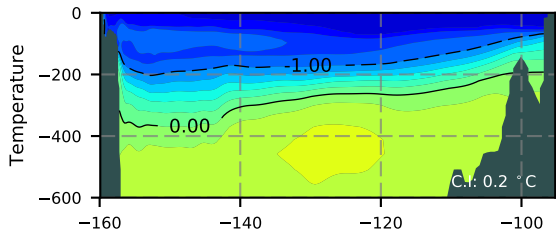
BCTGE28ERA5SC1BDY / Beaufort Section 1994
