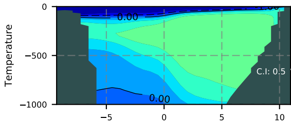
BCTGE28ERA5SC1BDY / FramS Section 1988
