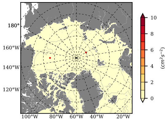
BCTGE28ERA5SC1EMP mean EKE @ 0 m over 1979
