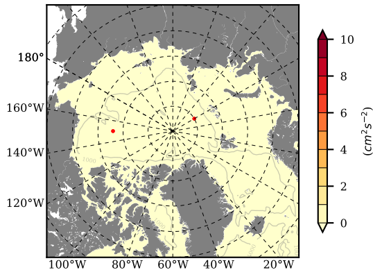
BCTGE28ERA5SC1EMP mean EKE @ 0 m over 1987
