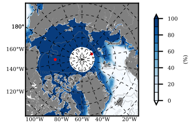
NSIDC mean SICON m09 1984
