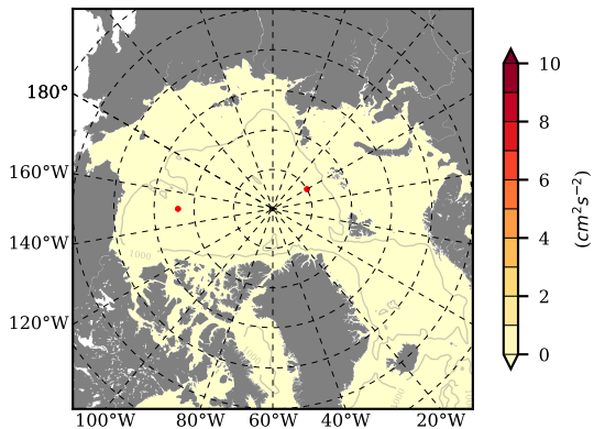
BCTGE28SS mean EKE @ 0 m over 2002
