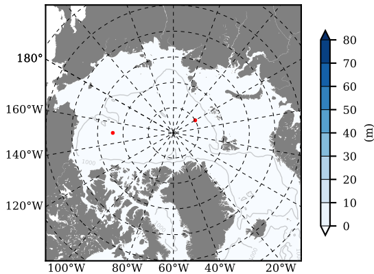
BCTGE28SS mean MLD01 over 1999 m03
