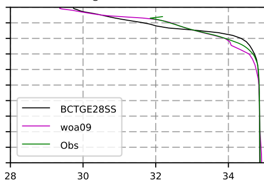
2014 mean Salinity @ moor Arctic B box
