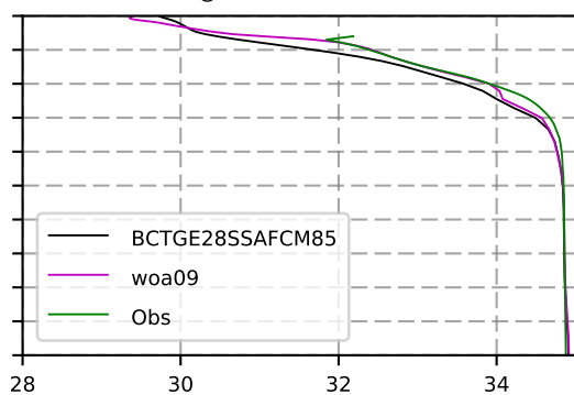
2042 mean Salinity @ moor Arctic B box
