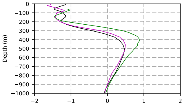
2046 mean temperature @ moor Arctic B box
