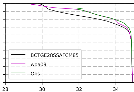
2046 mean Salinity @ moor Arctic B box
