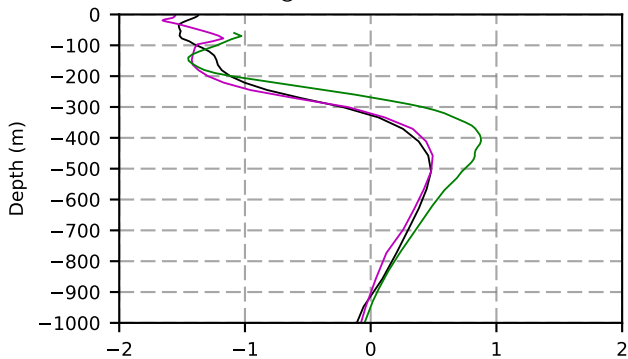
2052 mean temperature @ moor Arctic B box
