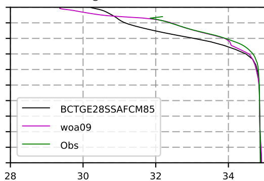
2052 mean Salinity @ moor Arctic B box
