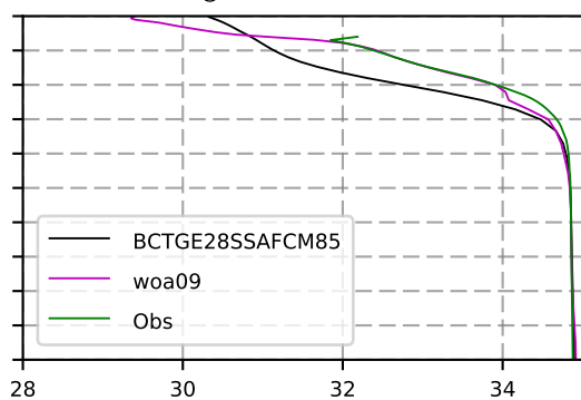
2057 mean Salinity @ moor Arctic B box
