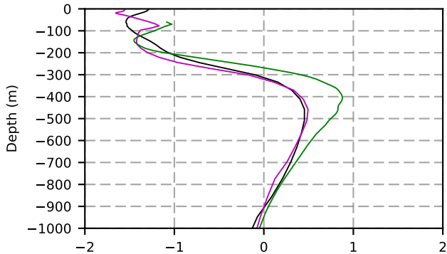
2059 mean temperature @ moor Arctic B box
