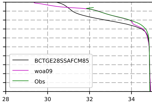
2059 mean Salinity @ moor Arctic B box
