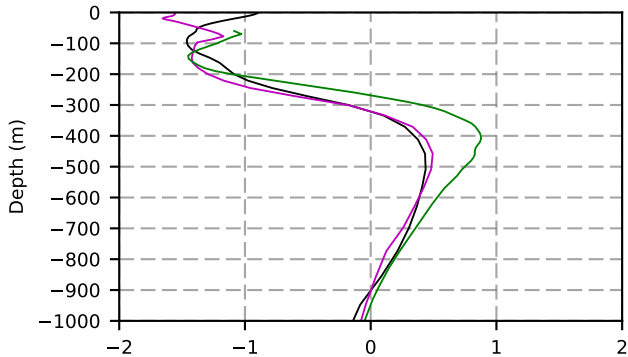
2060 mean temperature @ moor Arctic B box
