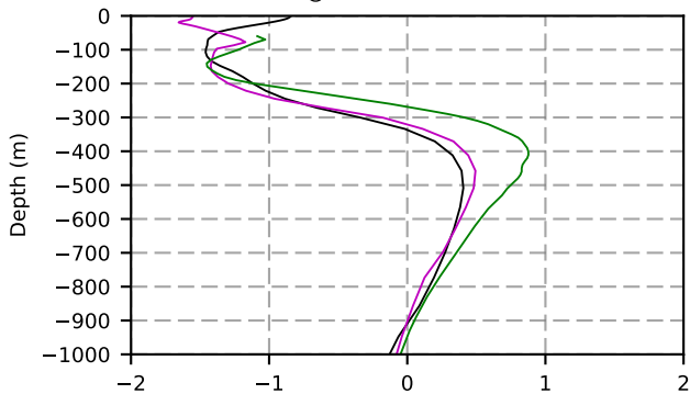
2064 mean temperature @ moor Arctic B box
