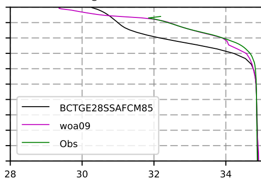
2064 mean Salinity @ moor Arctic B box
