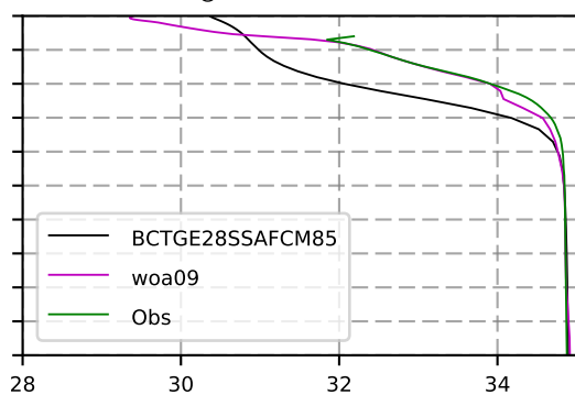
2066 mean Salinity @ moor Arctic B box
