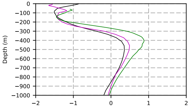
2068 mean temperature @ moor Arctic B box
