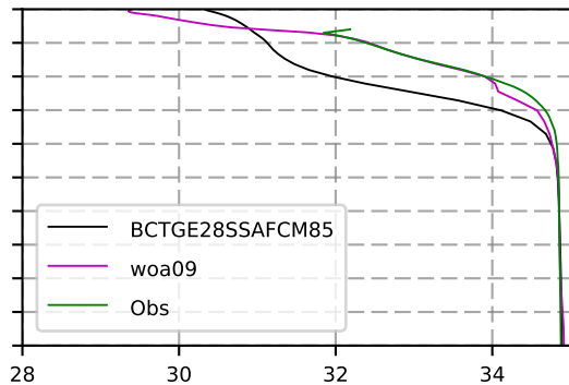
2069 mean Salinity @ moor Arctic B box
