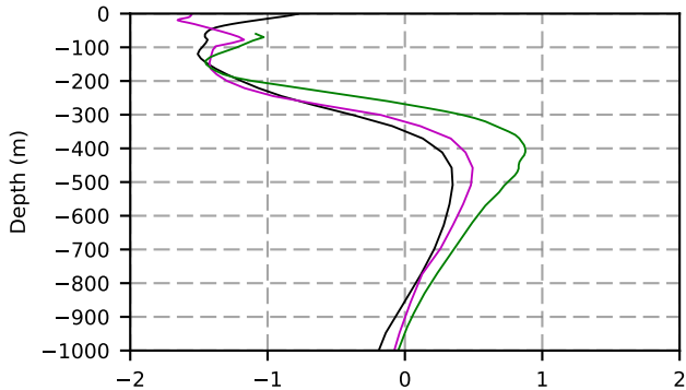
2069 mean temperature @ moor Arctic B box
