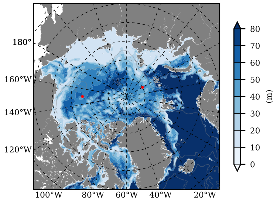
BCTGE28SSBDY mean MLD01 over 1986 m03
