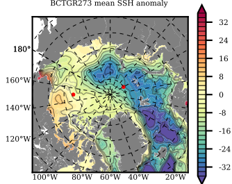
BCTGR273 mean SSH anomaly
