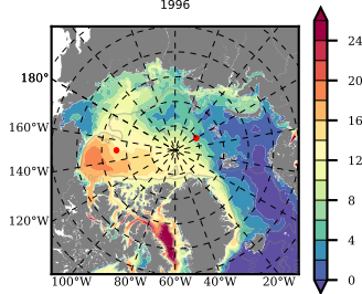
BCTGR273 mean FWC (m) over 1996
