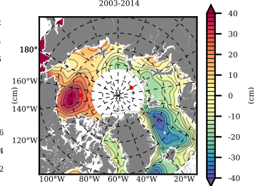
Mean DOT from Armitage et al. 2017 2003-2014
