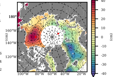
Mean DOT from Armitage et al. 2017 2013
