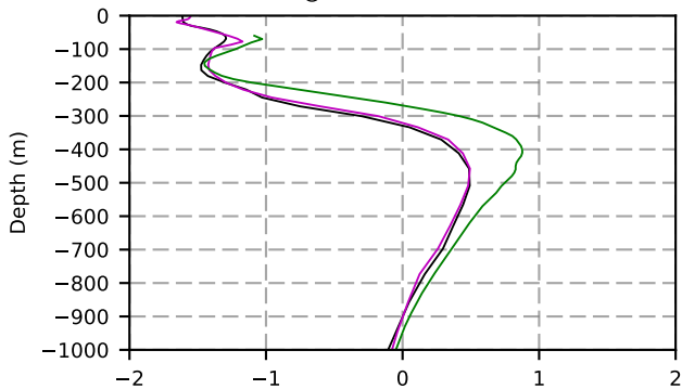
1980 mean temperature @ moor Arctic B box
