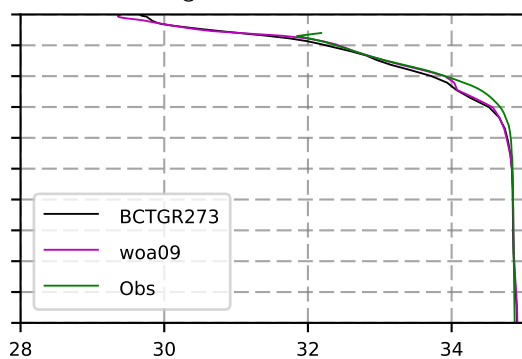
1980 mean Salinity @ moor Arctic B box
