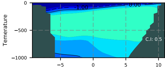
BCTGR273 / FramS Section 1981
