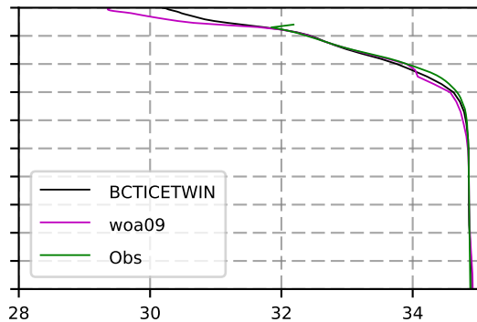
1993 mean Salinity @ moor Arctic B box
