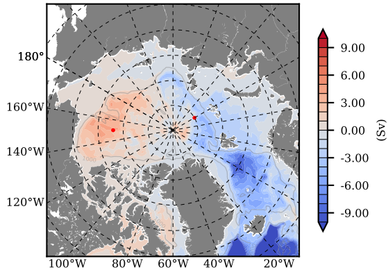
mean PSI over 1981
