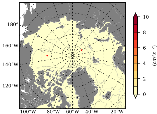
ERA01 mean EKE @ 0 m over 1985
