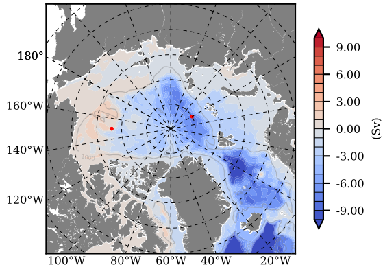
mean PSI over 1991
