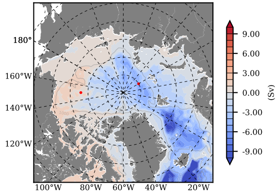
mean PSI over 1996
