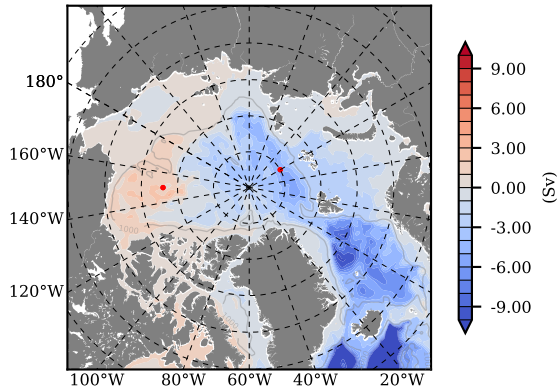
mean PSI over 1997
