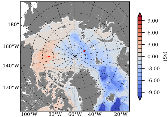
mean PSI over 1998
