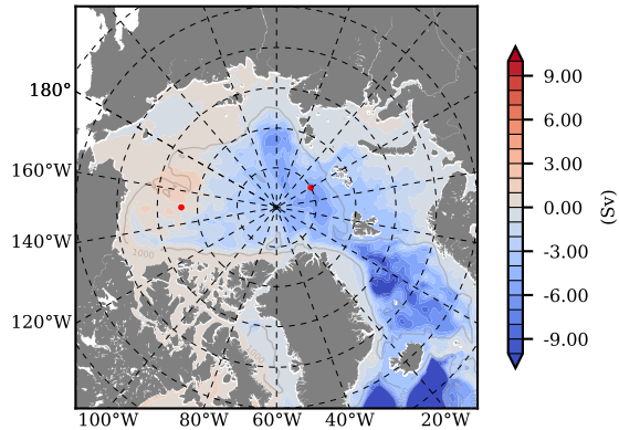
mean PSI over 2006
