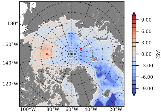
mean PSI over 2008
