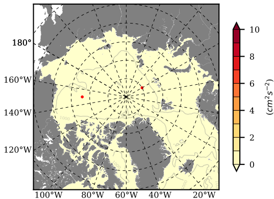
ERA01 mean EKE @ 0 m over 2009
