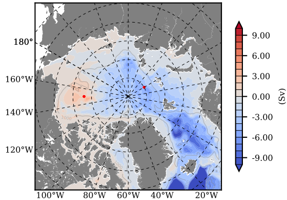
mean PSI over 2009
