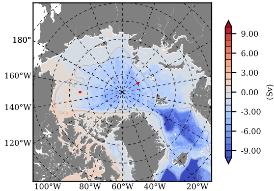
mean PSI over 2016
