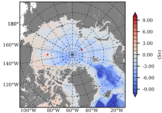
mean PSI over 2018
