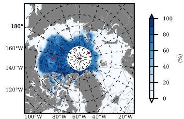
NSIDC mean SICON m09 1990
