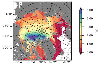
NSIDC mean SICON m03 1990
