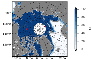
NSIDC mean SICON m09 2007
